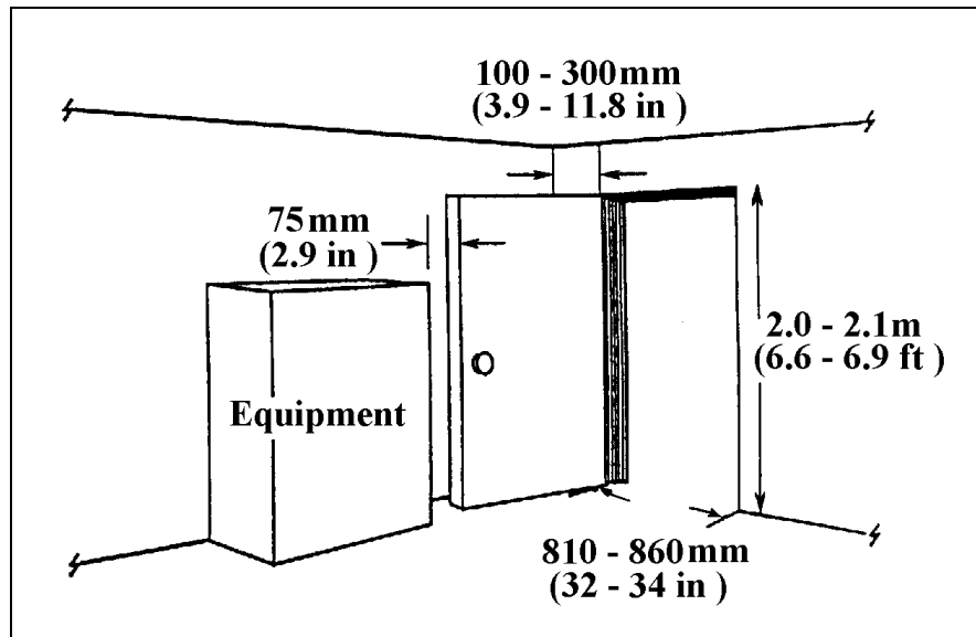
Exhibit 9.3.4.2.1 Door dimensions
