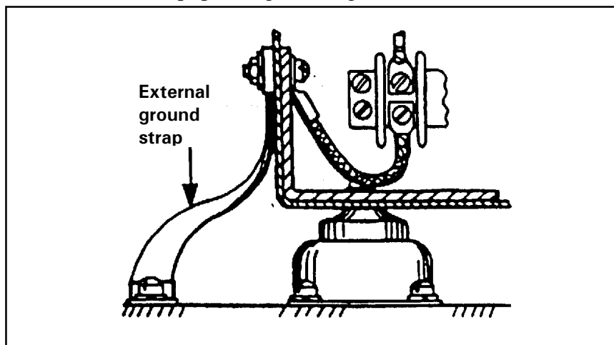
Exhibit 12.4.4.6 Equipment grounding
